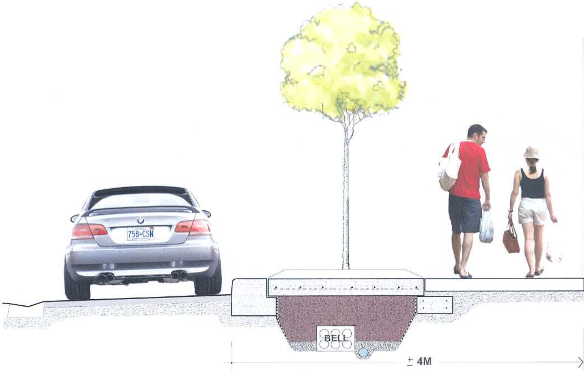
section through continuous soil trench
